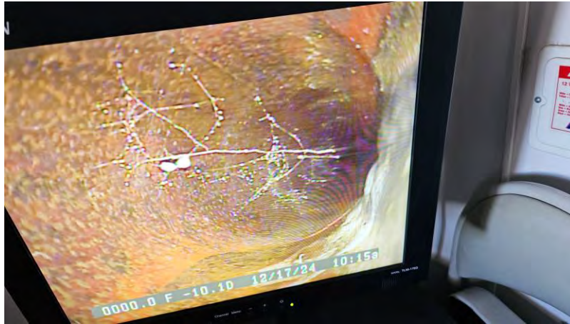
Main wastewater line on Copper Drive. Full of cobwebs that block the camera
